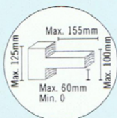
Straight Shoulder Tenon
