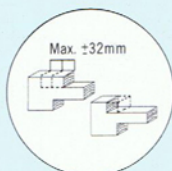
Staggered Tenon
